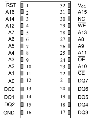
32-Pin Encapsulated Package 740mil Flush
